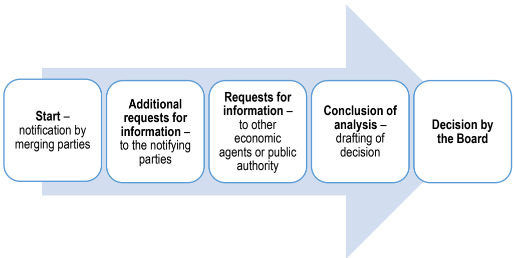
Figure 10. Merger process
